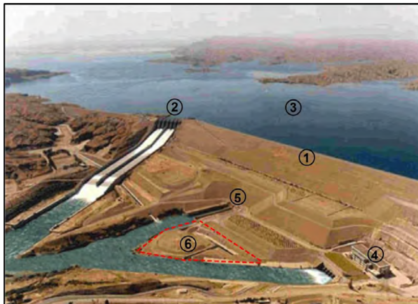
Fig. 1 General plan of the Karkheh dam project. The numbers represent: 1, dam crest; 2, spillway; 3, reservoir; 4, powerhouse; 5, diversion culverts; and 6, the location of the new relief wells at dam toe (the red-dashed polygon)
