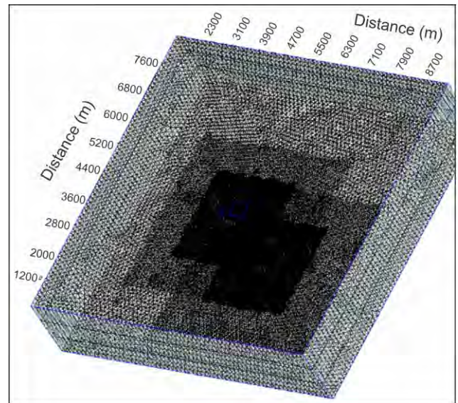
Fig. 7 Computational 3D mesh used for modeling the artesian aquifer confined between mudstone layers (-3) and (-2) at the Karkheh dam toe
